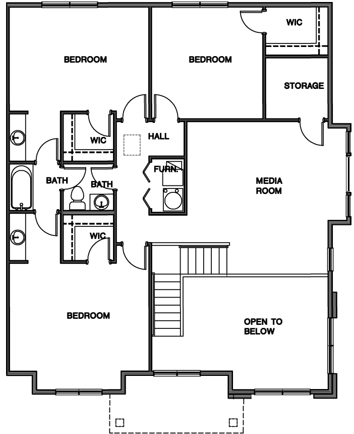
LEVEL TWO - 1,236 SQ FT
