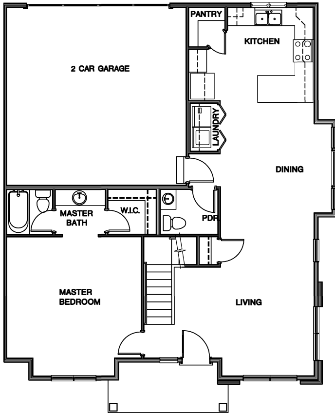
LEVEL ONE - 1,052 SQ FT
